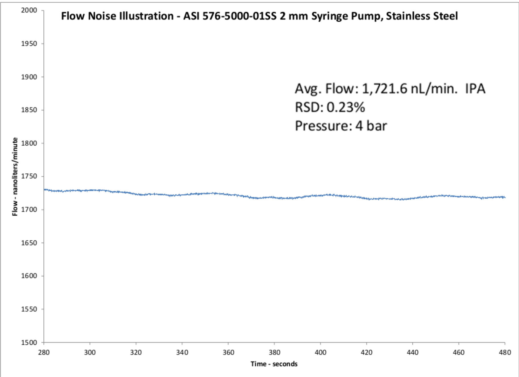
ASI at 4 bar
