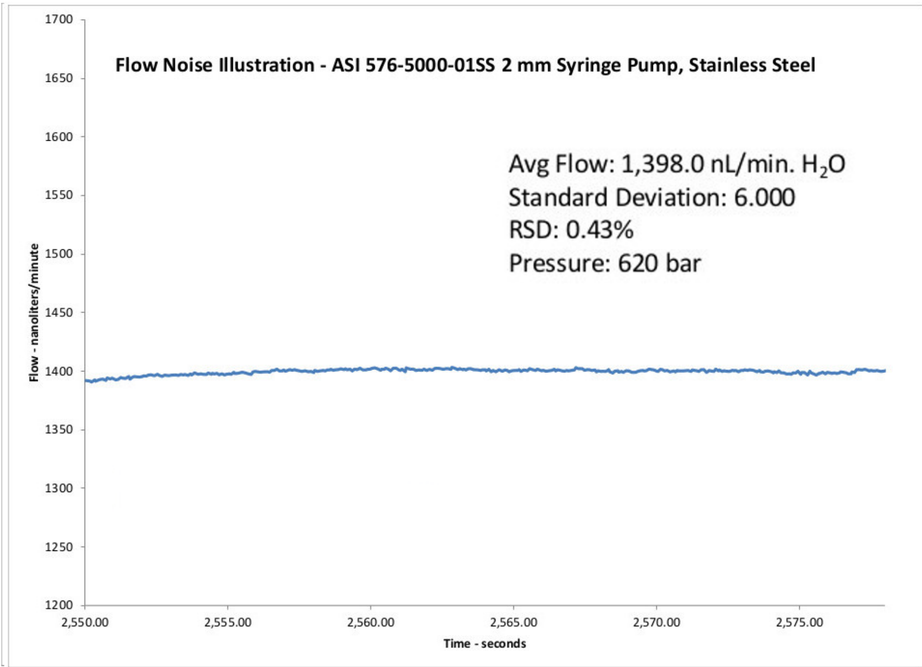
ASI at 620 bar
